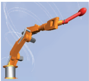
Animation of a detailed model of a robot built with the MultiBody package in the Modelica Standard library
